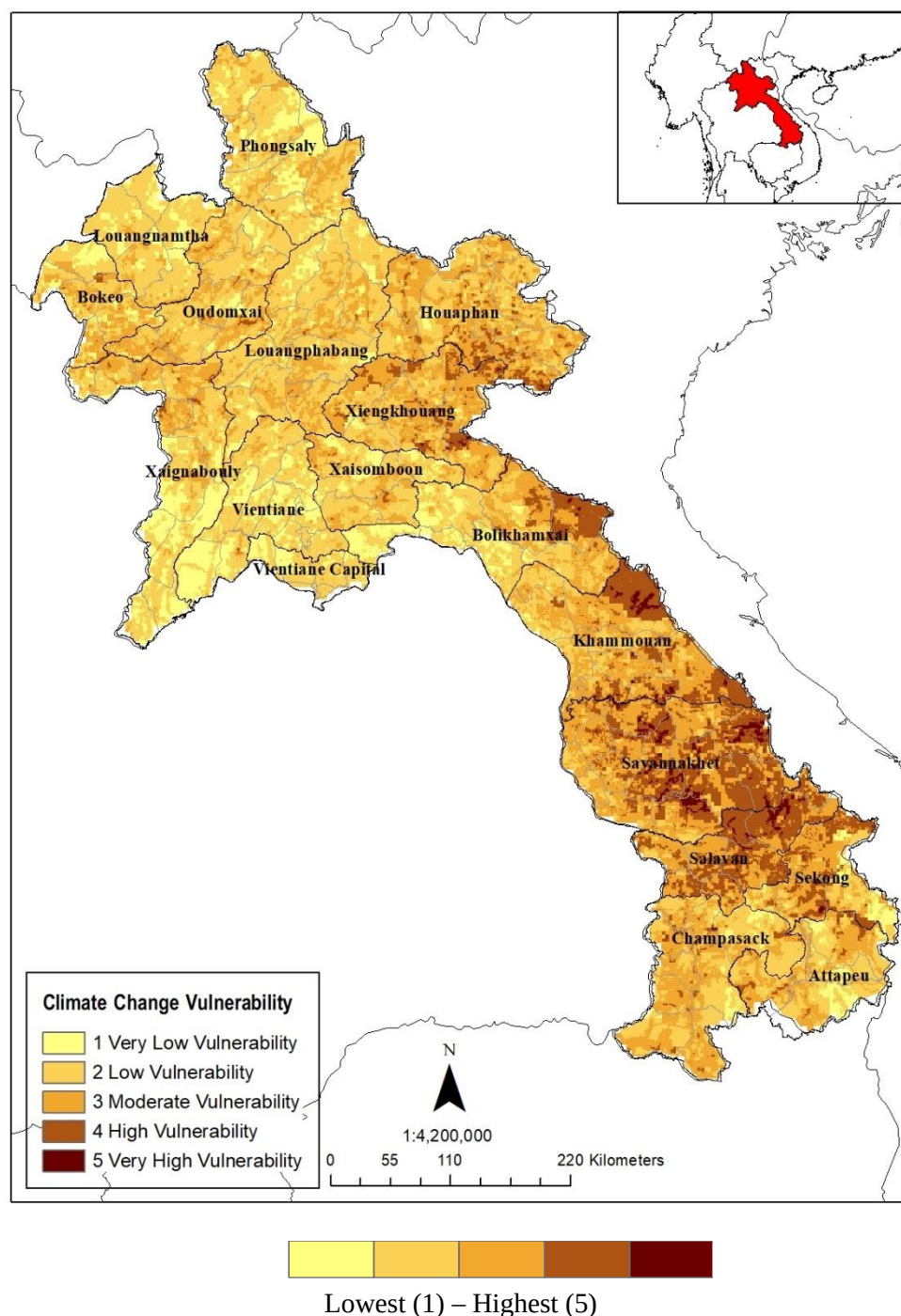
Figure 36: Climate change vulnerability map of Lao PDR
