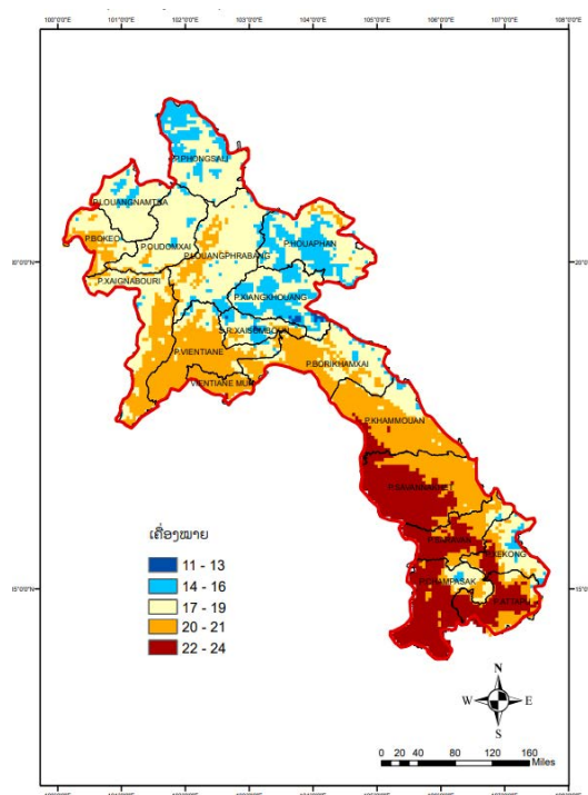
Figure 15: Min temperature trend over the next 30 years
